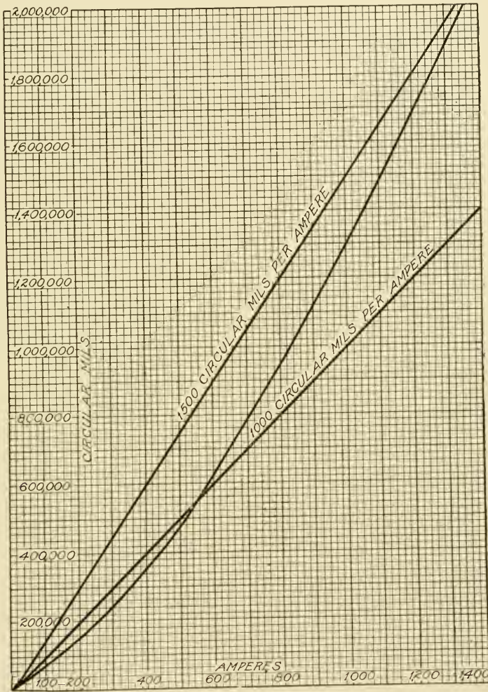
Fig. 2. Curves Showing Safe Carrying Capacity of Copper Wires
